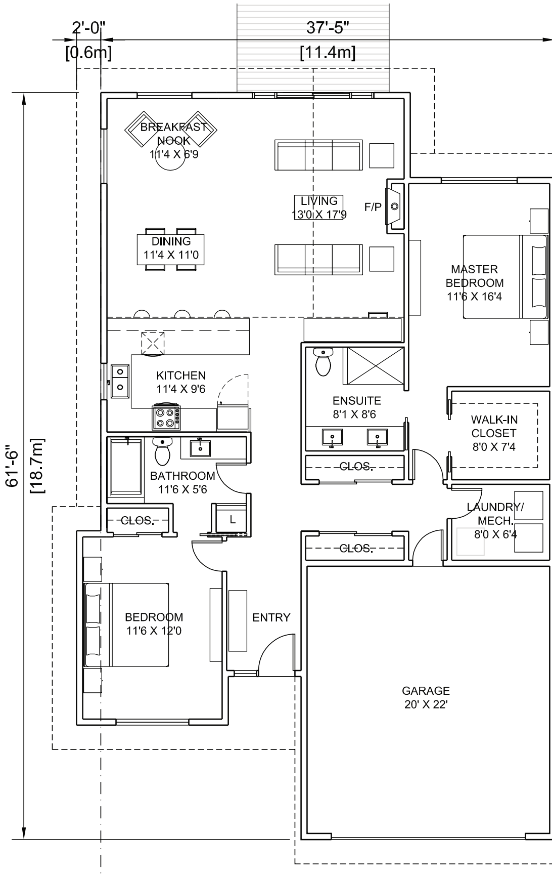
TYPE 4 - RANCHER TWO BEDROOM 1605 SF (END UNIT)
